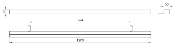
Dimensions [mm]
