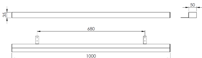
Dimensions [mm]
